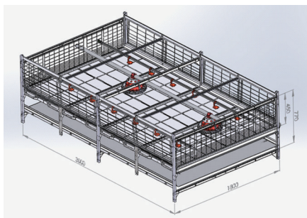
Broiler Cage 3000×1800
